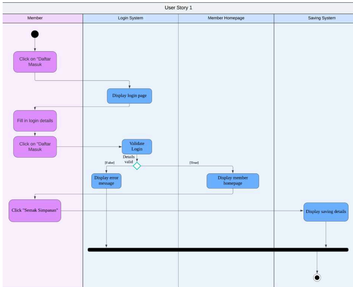
Figure 9: Activity Diagram for <<Name of User Story>>
