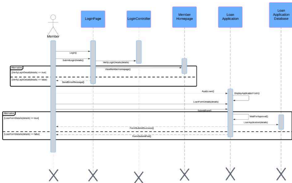
Figure 5: Sequence Diagram for <Name of User Story/Scenario if more than one scenario>
