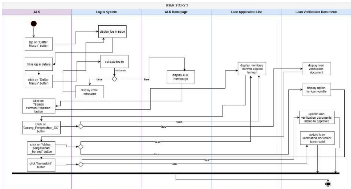
Figure 2.5: Activity Diagram for ALK approved loan application
