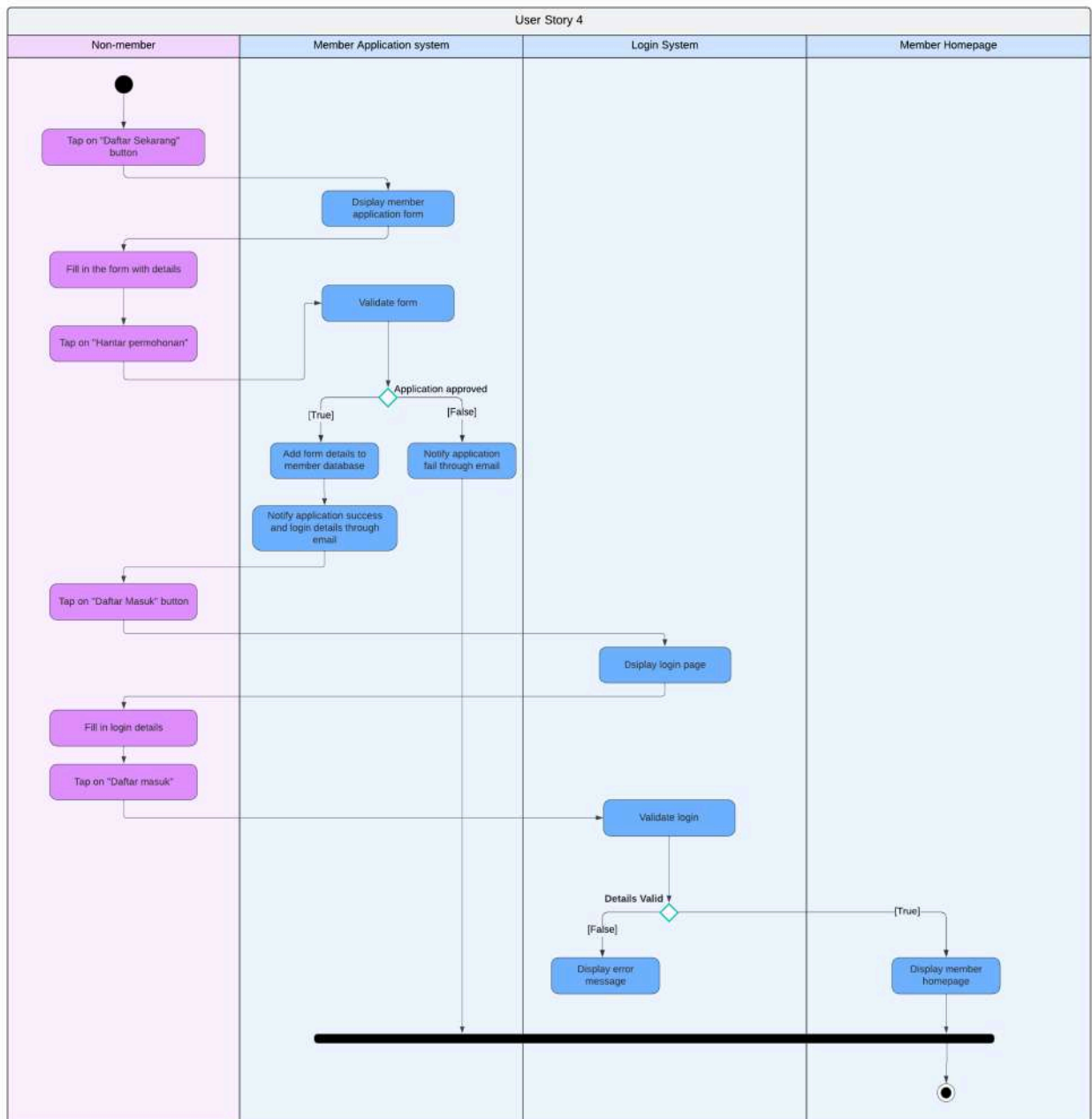
Figure 2.2: Activity Diagram for US004 User Story
