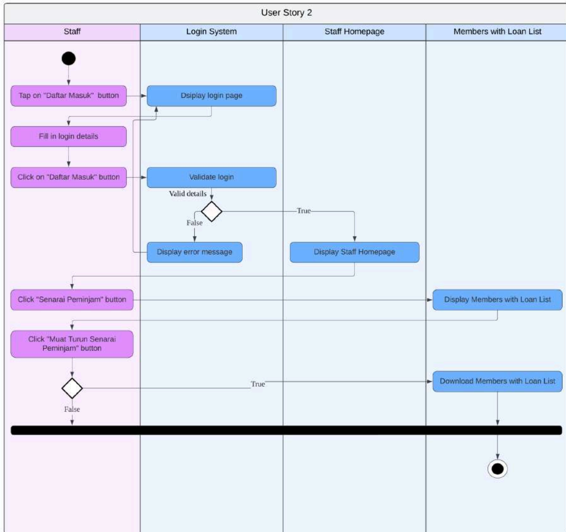
Figure 13: Activity Diagram for when Staff Chooses to View Members with Loan List
