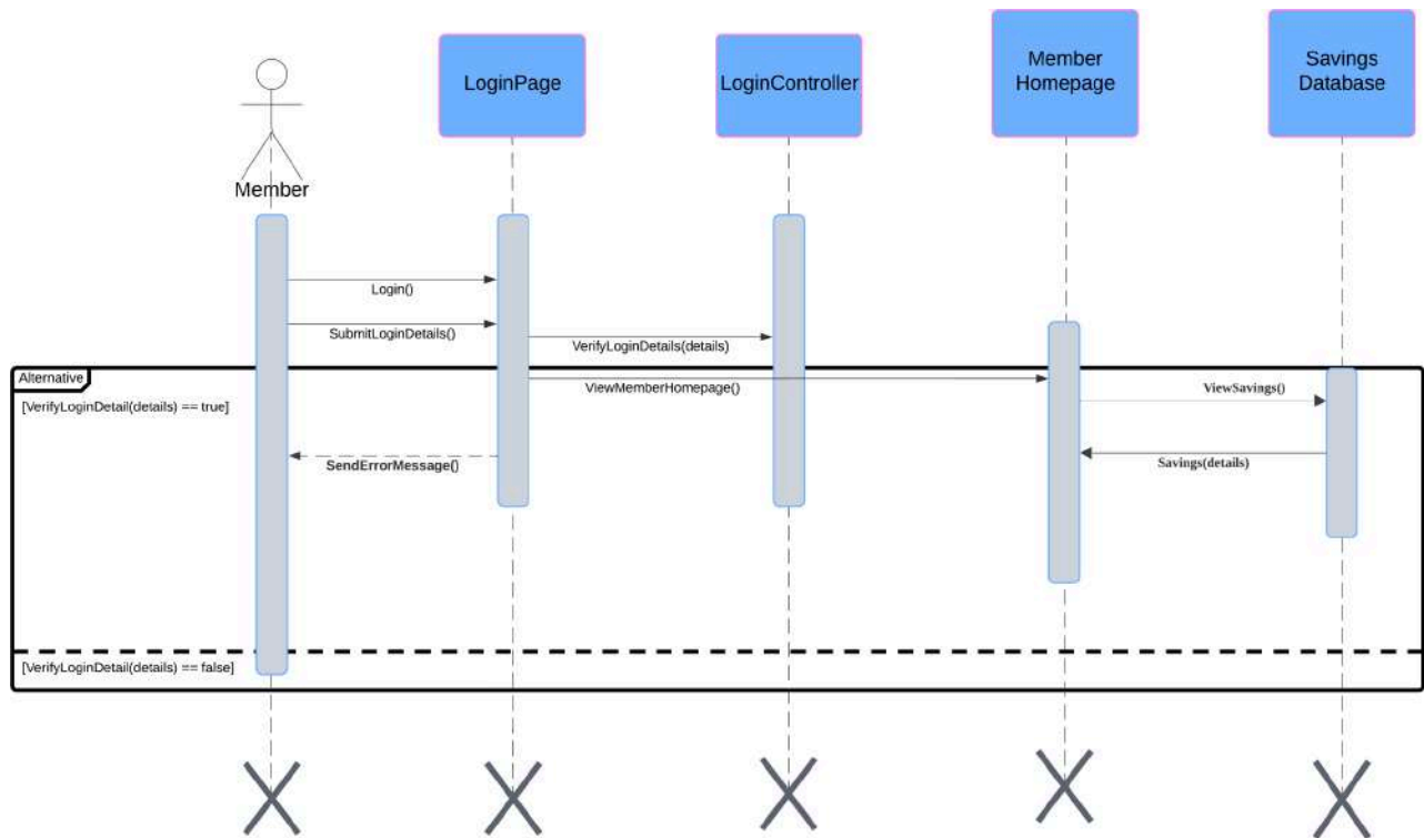
Figure 5: Sequence Diagram for <Name of User Story/Scenario if more than one scenario>
