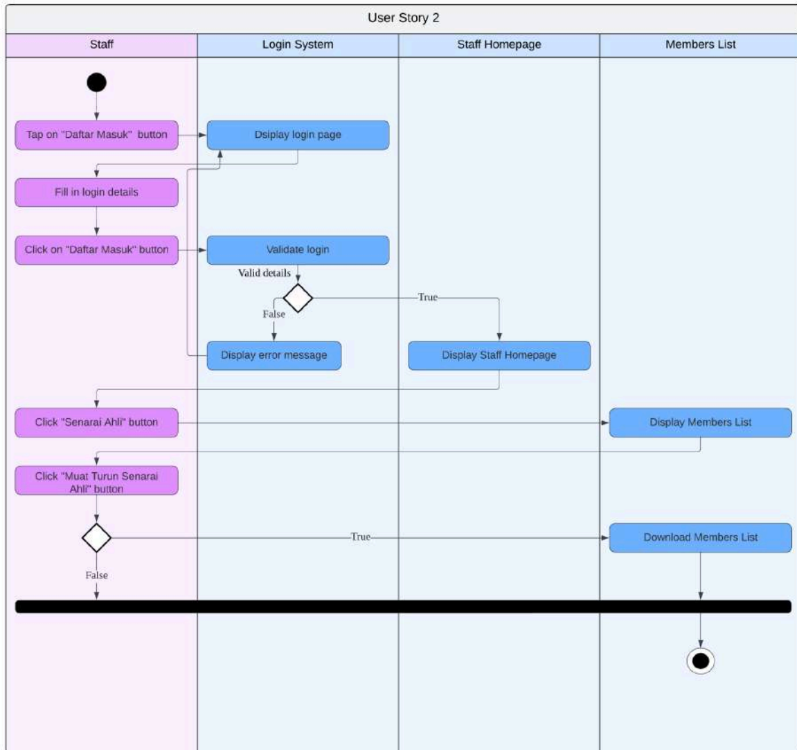
Figure 12: Activity Diagram for when Staff Chooses to View Members List
