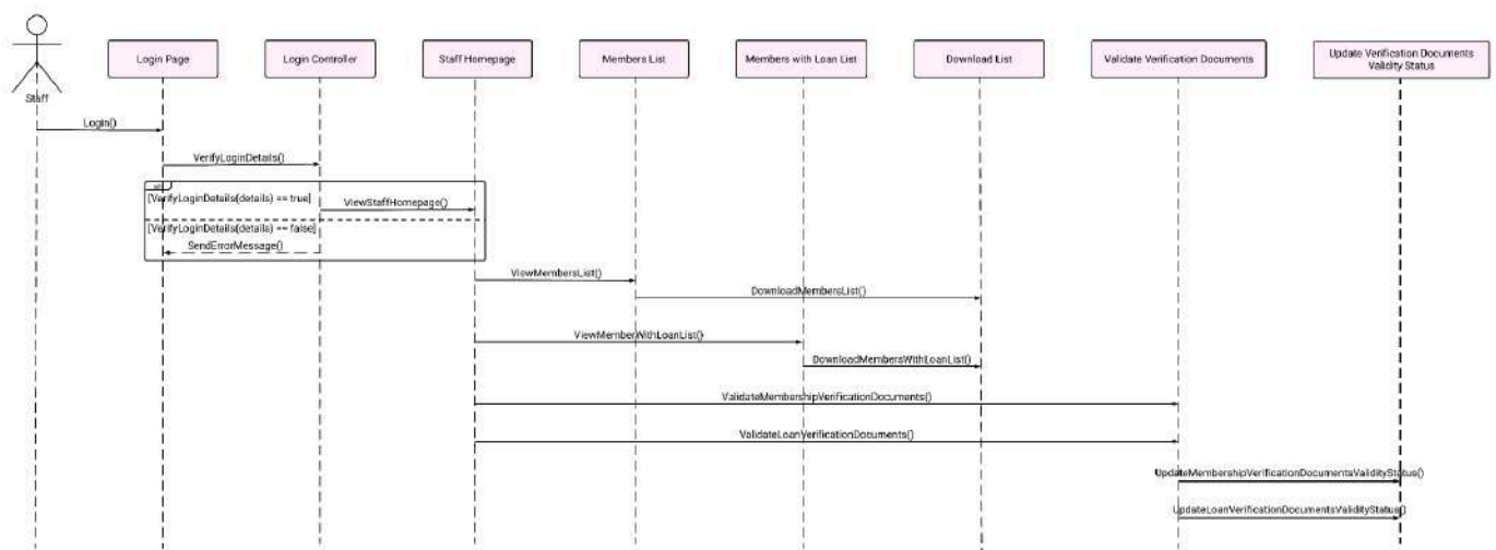
Figure 11: Sequence Diagram for US002 User Story
