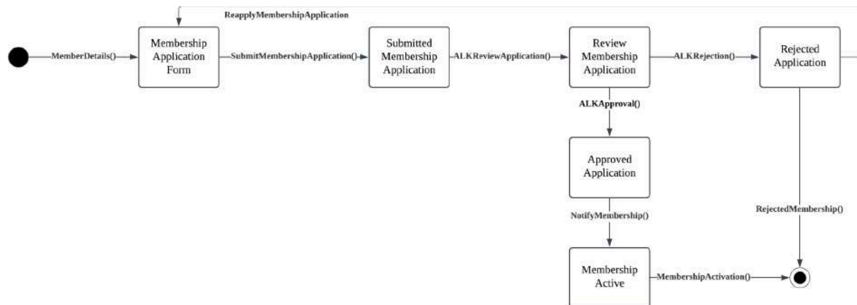
Figure 3: State Machine Diagram for <Name of the System> - syah
