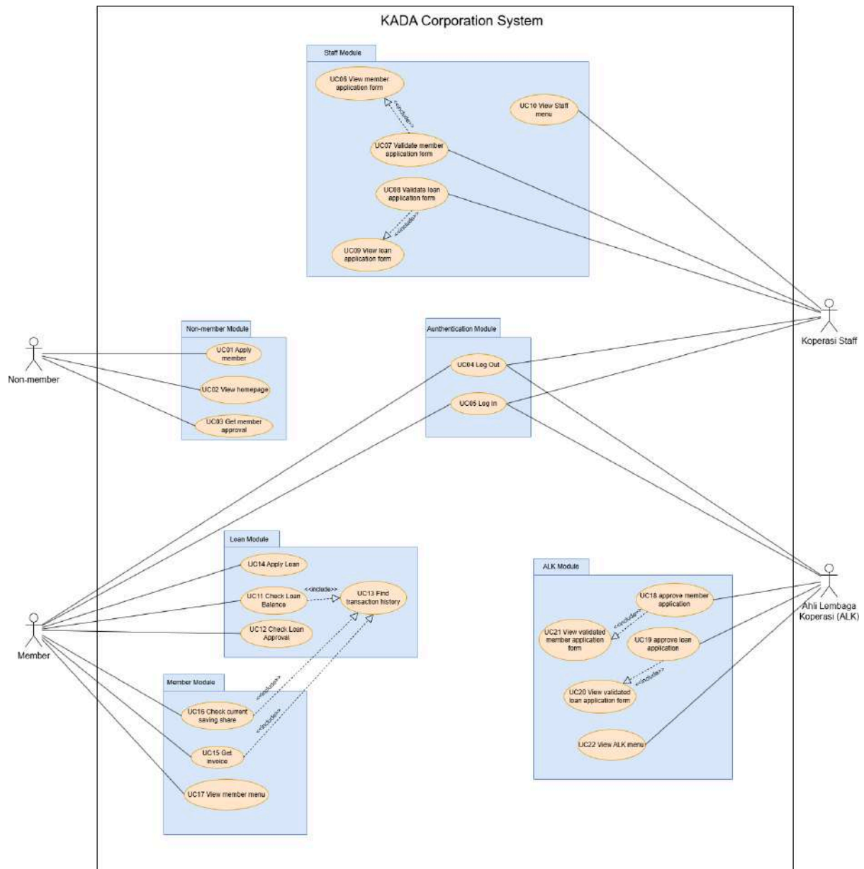
Figure 1: Use Case Diagram for KADA Corporation System
