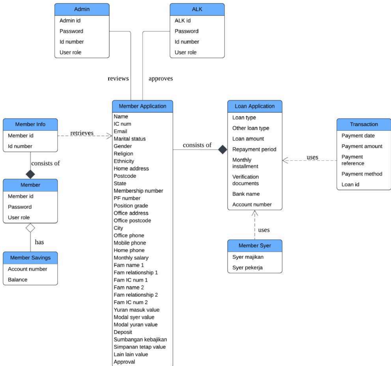
Figure 2: Domain Model for Koperasi KADA system
