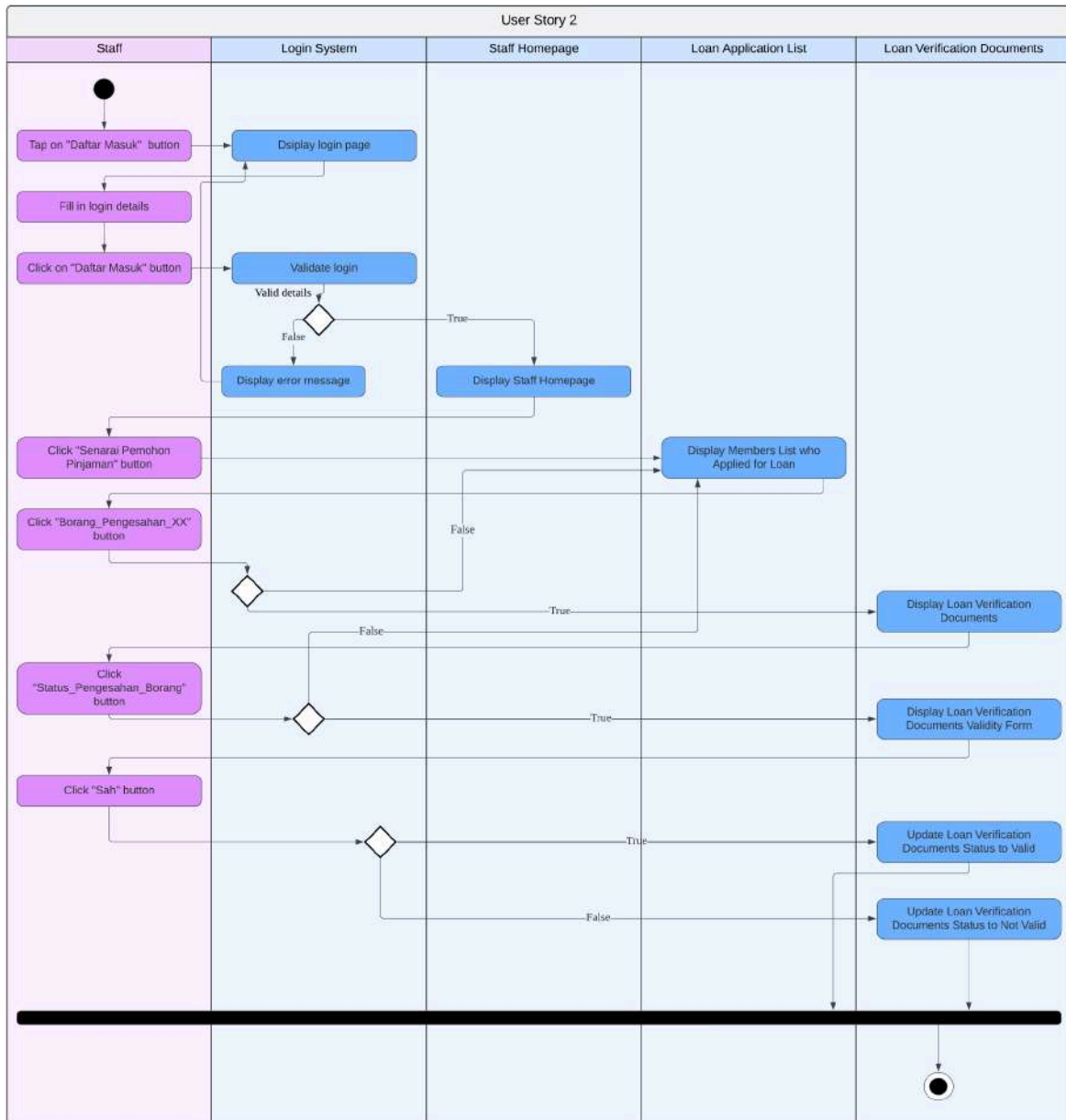
Figure 15: Activity Diagram for when Staff Chooses to View Loan Application List by Members
