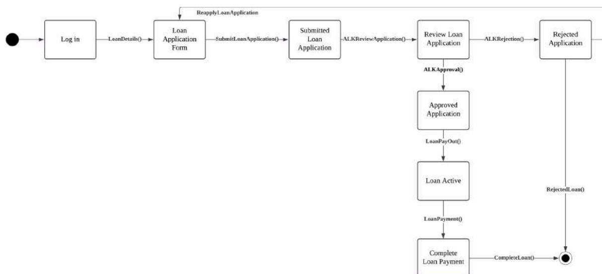
Figure 4: State Machine Diagram for <Name of the System> - syah
