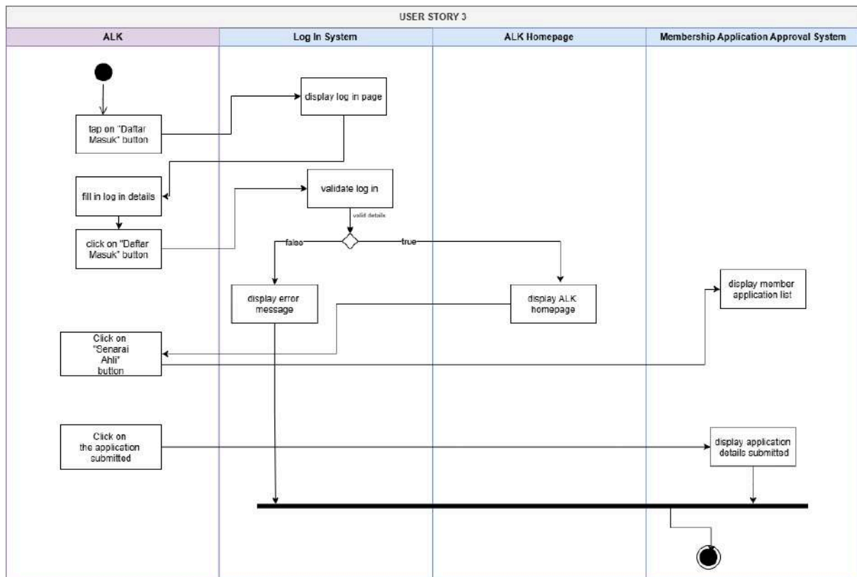
Figure 2.5: Activity Diagram for ALK view validated member application
