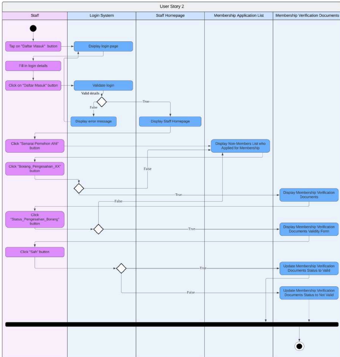
Figure 14: Activity Diagram for when Staff Chooses to View Membership Application List by Non-Members
