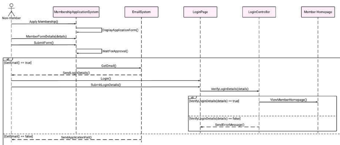
Figure 2.5: Sequence Diagram for US004 User Story
