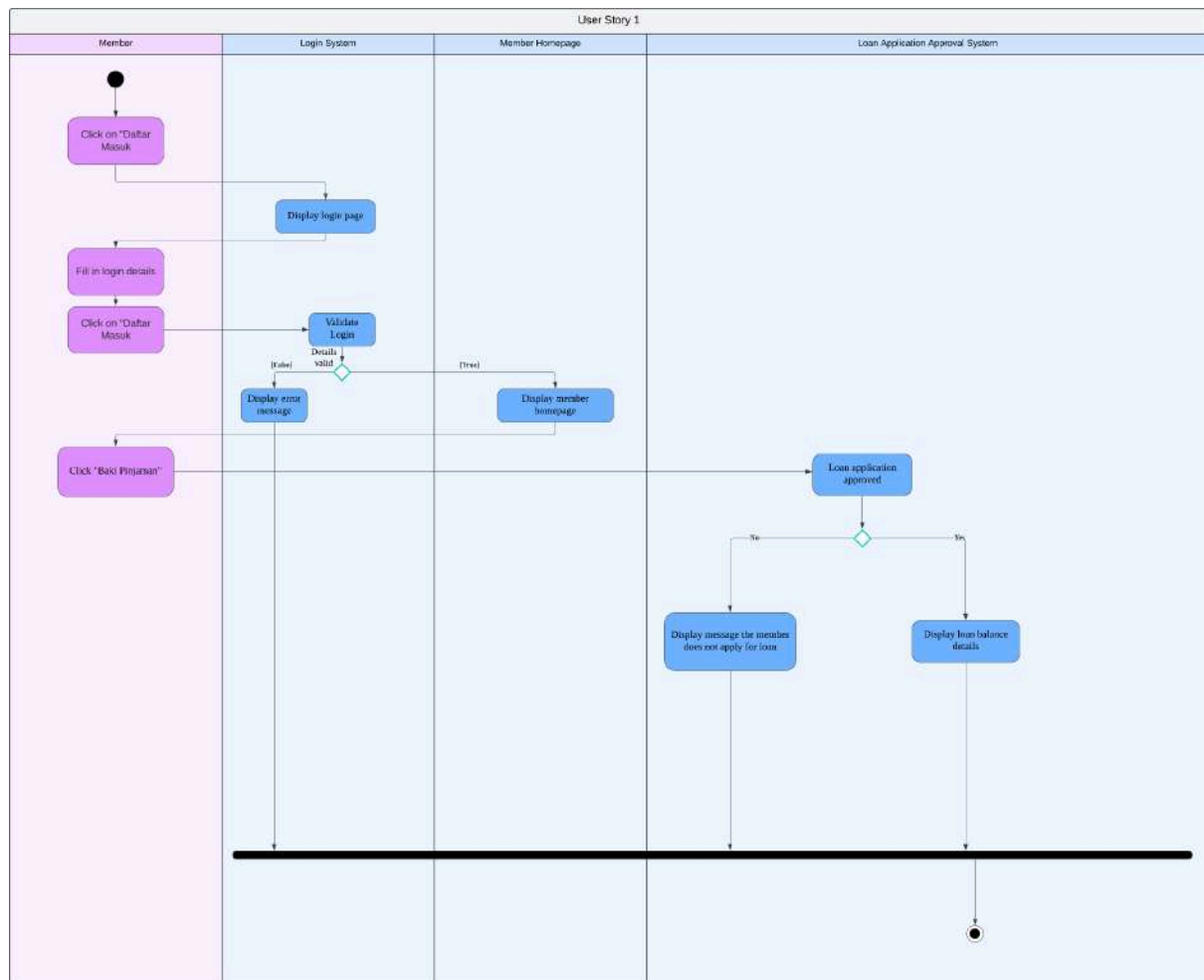
Figure 8: Activity Diagram for <<Name of User Story>>
