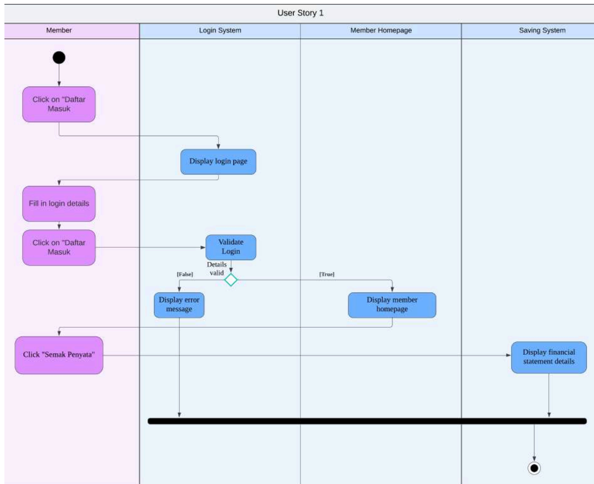
Figure 10: Activity Diagram for <<Name of User Story>>
