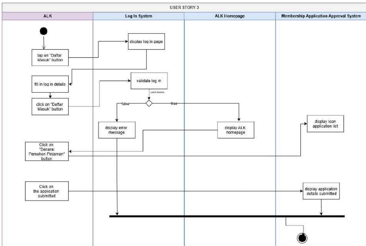
Figure 2.5: Activity Diagram for ALK view validated loan application
