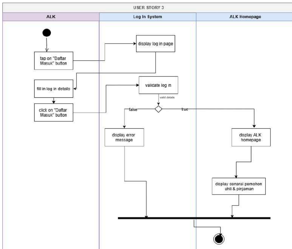
Figure 2.5: Activity Diagram for view ALK menu
